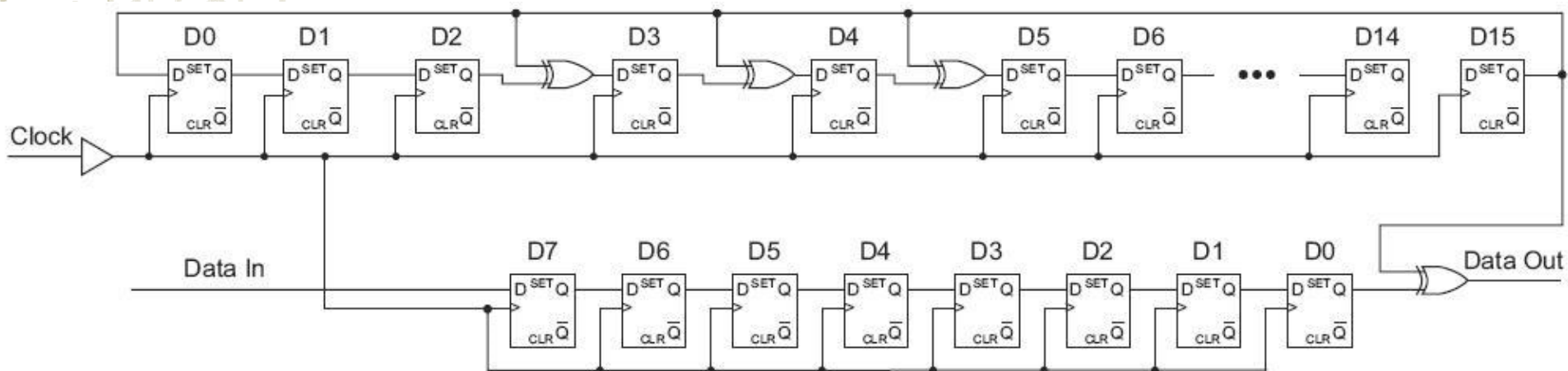
LFSR skrembler
